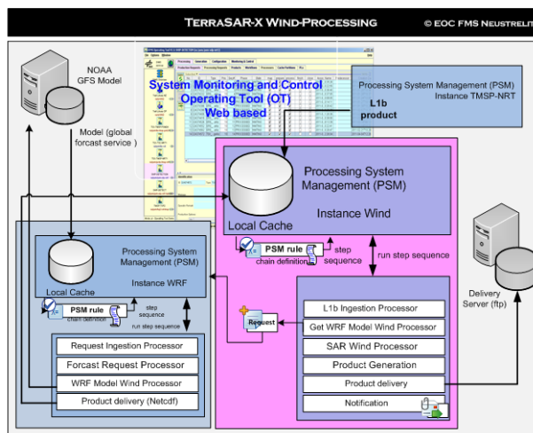
Figure 5. TerraSAR-X NRT wind processing work flow
